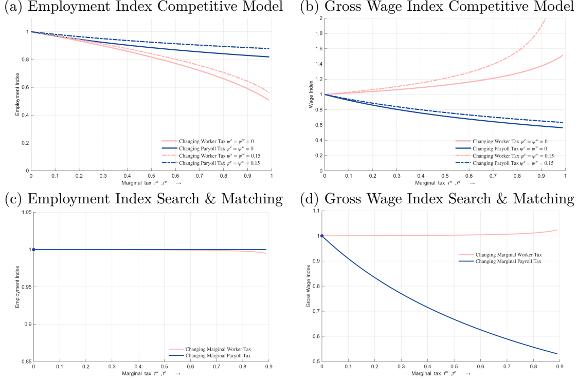
Figure K.1. : Effect on employment and gross wages of varying marginal tax rates
